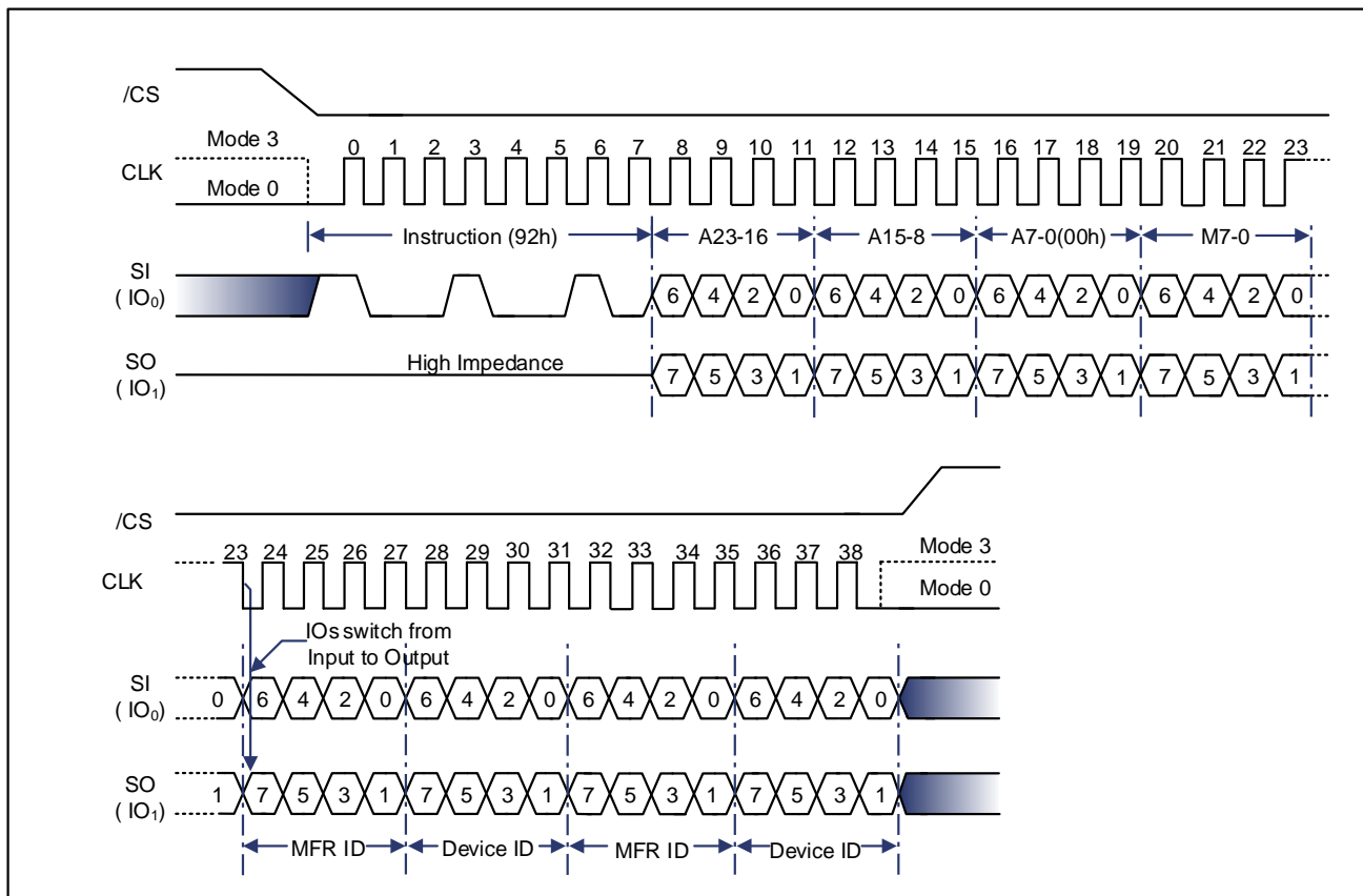
Figure 9-67 Read Manufacturer / Device ID Dual I/O Instruction (SPI Mode only)
