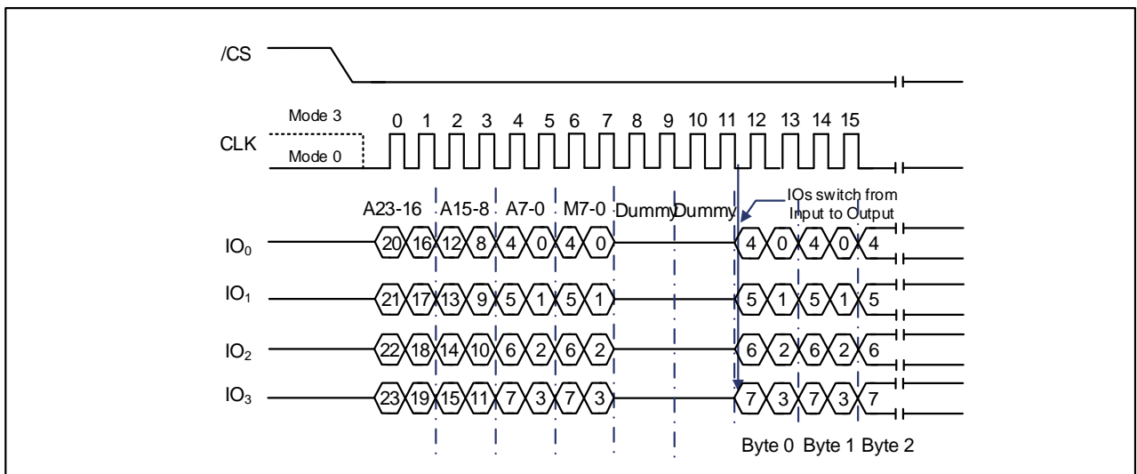
Figure 9-34 Fast Read Quad I/O Instruction (Previous instruction set M5-4 = 10, SPI Mode)
