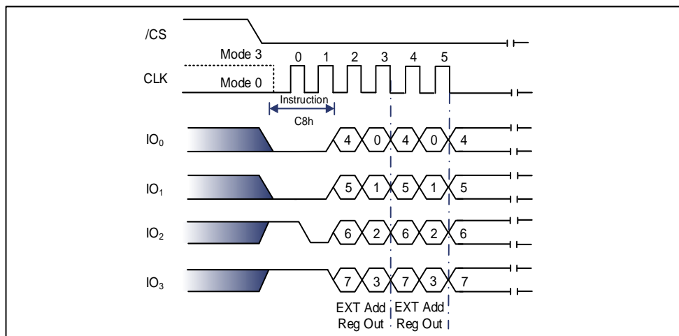
Figure 9-11 Read Extended Address Register Instruction (QPI Mode)
