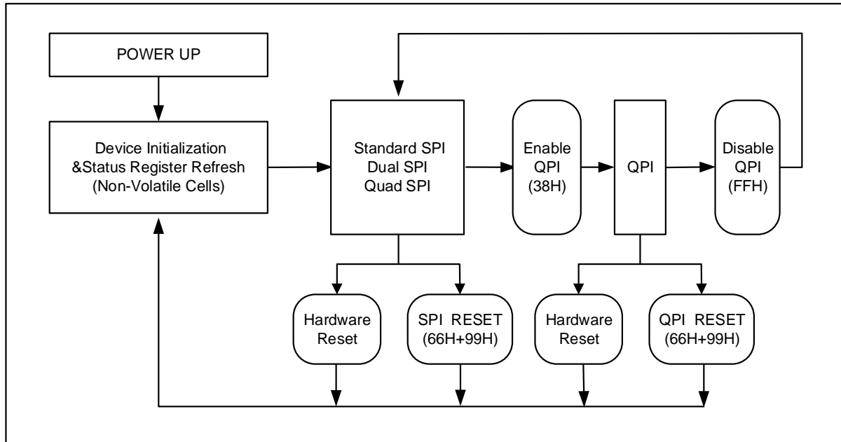
Figure 7-1 XM25QH01D Serial Flash Memory Operation Diagram
