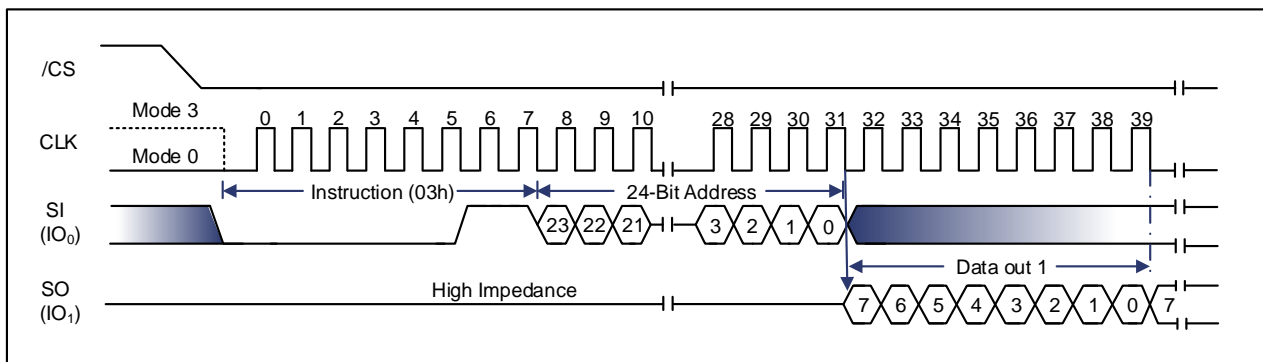
Figure 9-16 Read Data Instruction (SPI Mode only)
