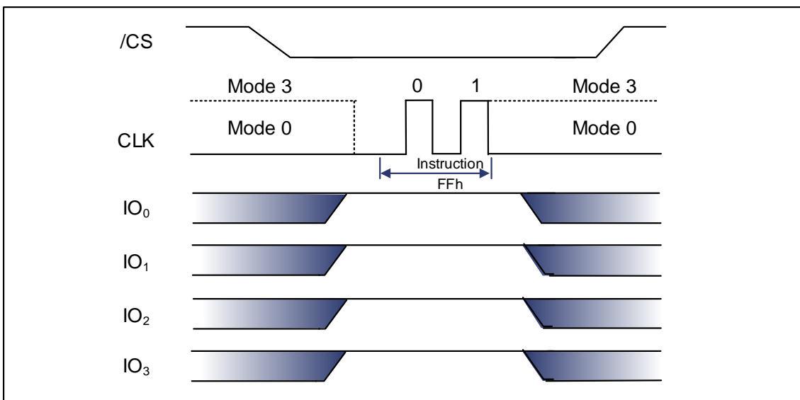
Figure 9-84 Exit QPI Instruction (QPI Mode only)
