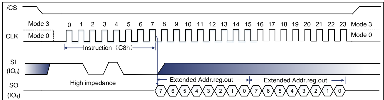
Figure 9-10 Read Extended Address Register Instruction (SPI Mode)
