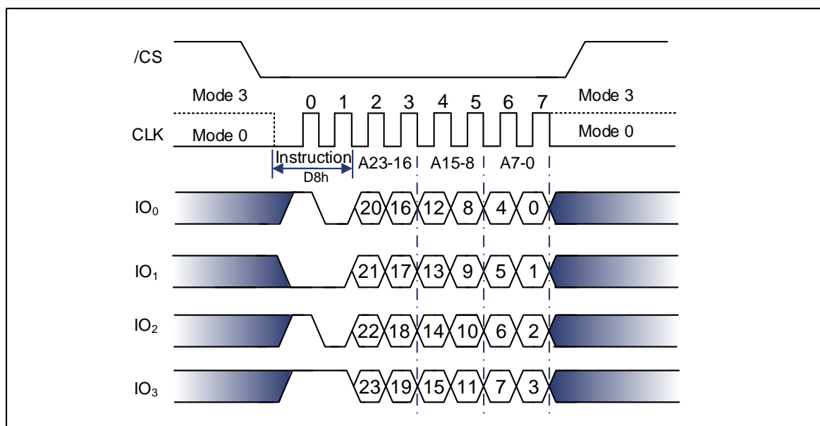
Figure 9-56 64KB Block Erase Instruction (QPI Mode)
