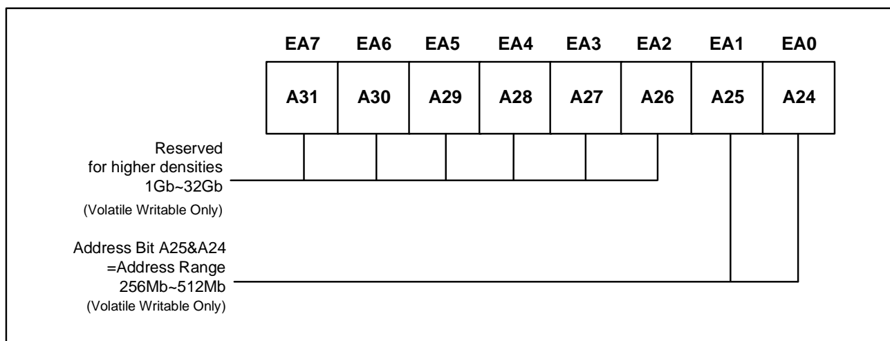
Figure 8-4 Extended Address Register
