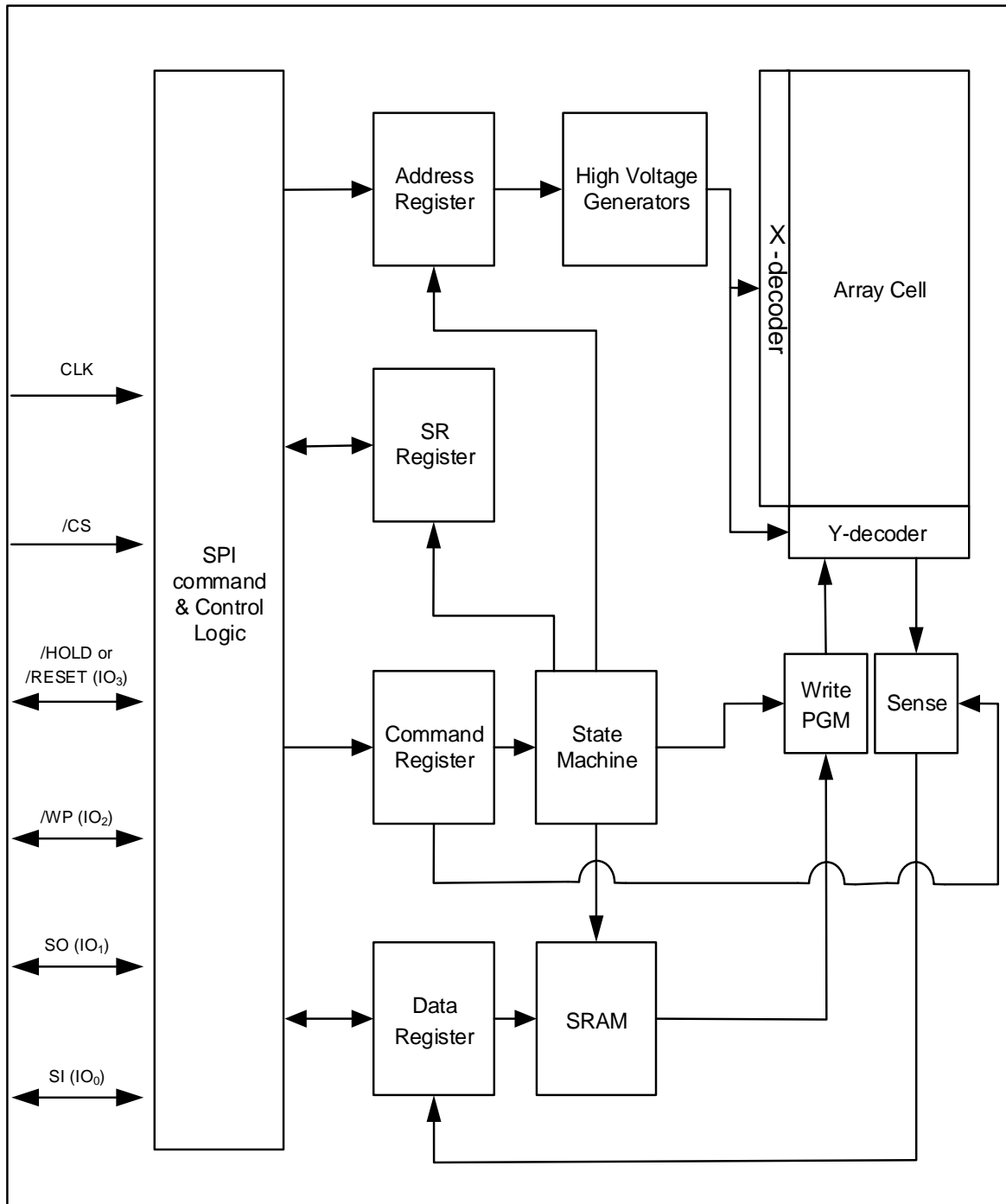
Figure 4-1 XM25QH01D Serial Flash Memory Block Diagram
