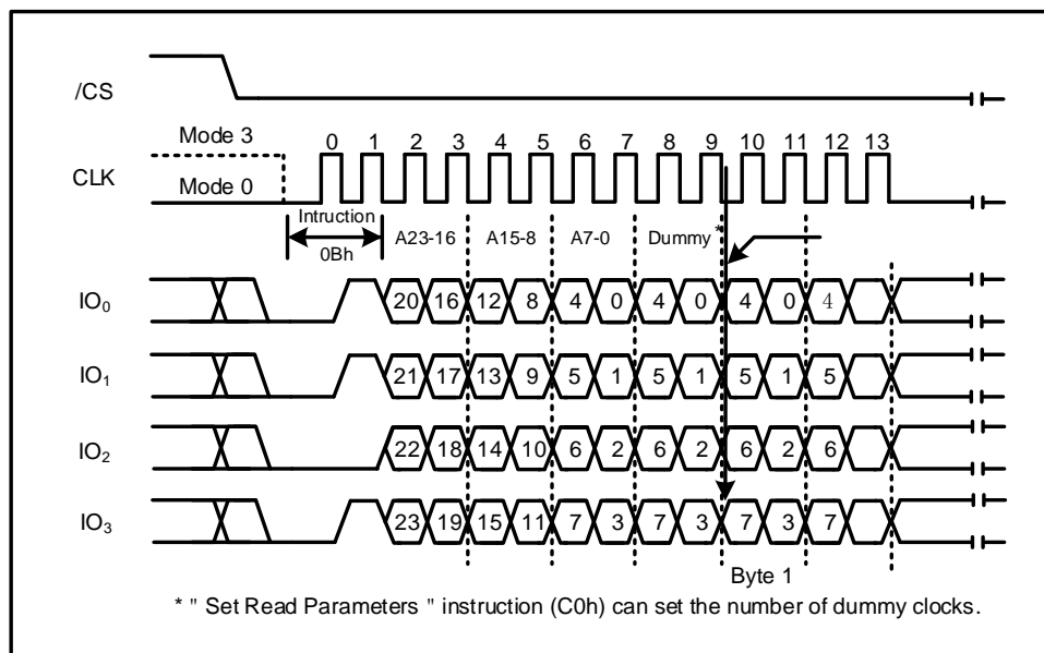
Figure 11b. Fast Read Instruction (QPI Mode)
