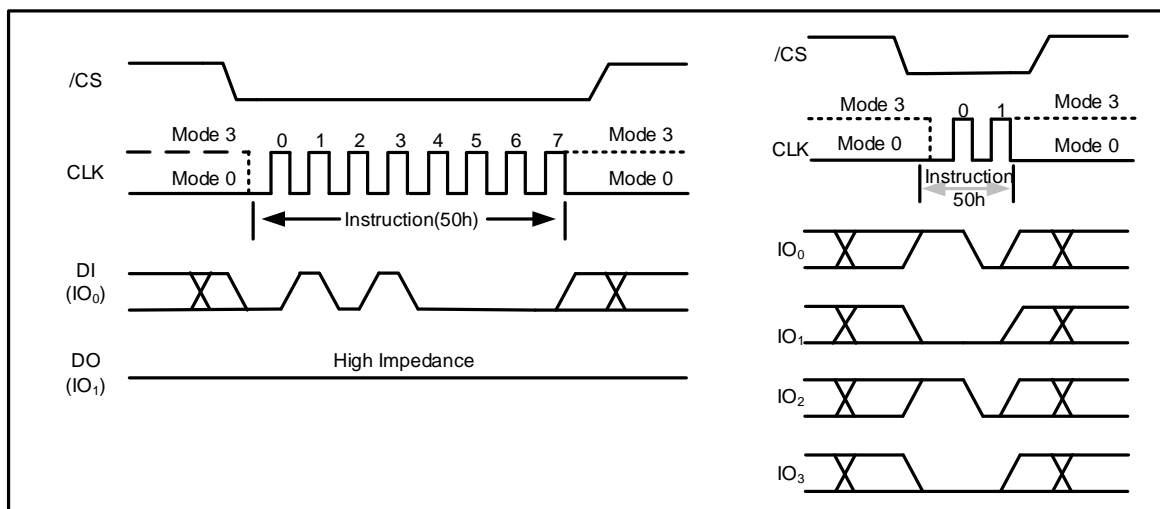
Figure 6. Write Enable for Volatile Status Register Instruction for SPI Mode (left) or QPI Mode (right)
