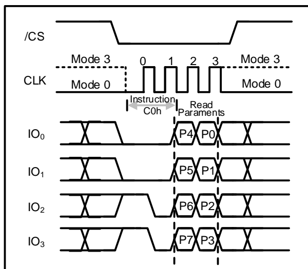
Figure 42. Set Read Parameters Instruction (QPI Mode only)
