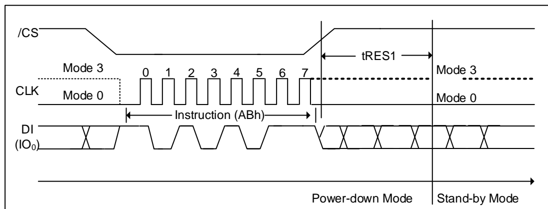
Figure 32a. Release Power-down Instruction (SPI Mode)
