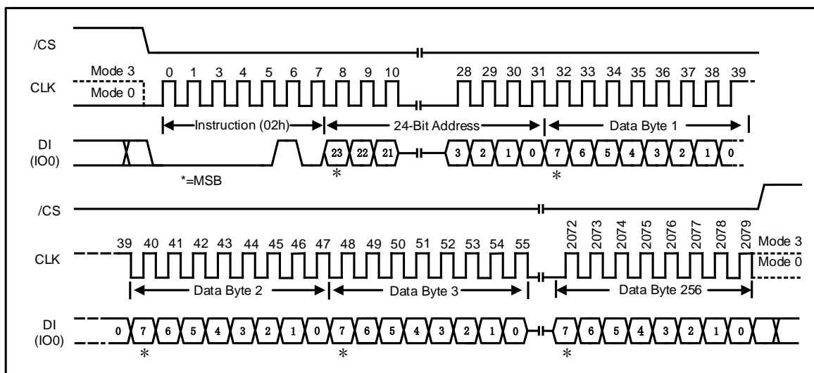
Figure 22a. Page Program Instruction (SPI Mode)
