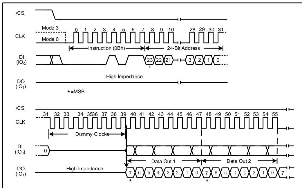
Figure 11a. Fast Read Instruction (SPI Mode)
