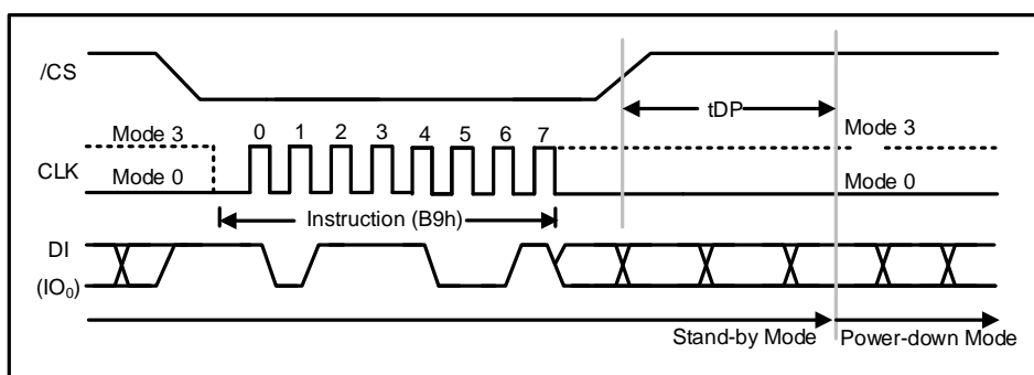
Figure 31a. Deep Power-down Instruction (SPI Mode)
