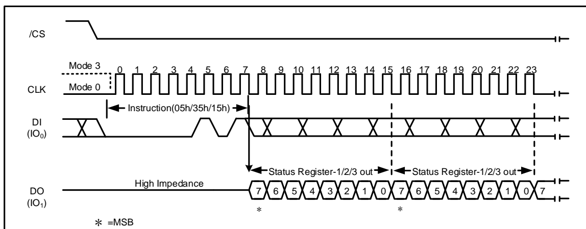
Figure 8a. Read Status Register Instruction (SPI Mode)
