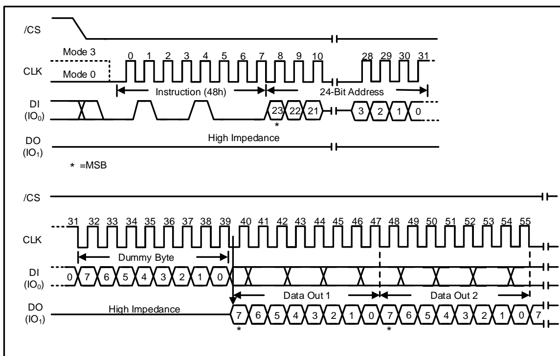
Figure 41. Read Security Registers Instruction (SPI Mode only)
