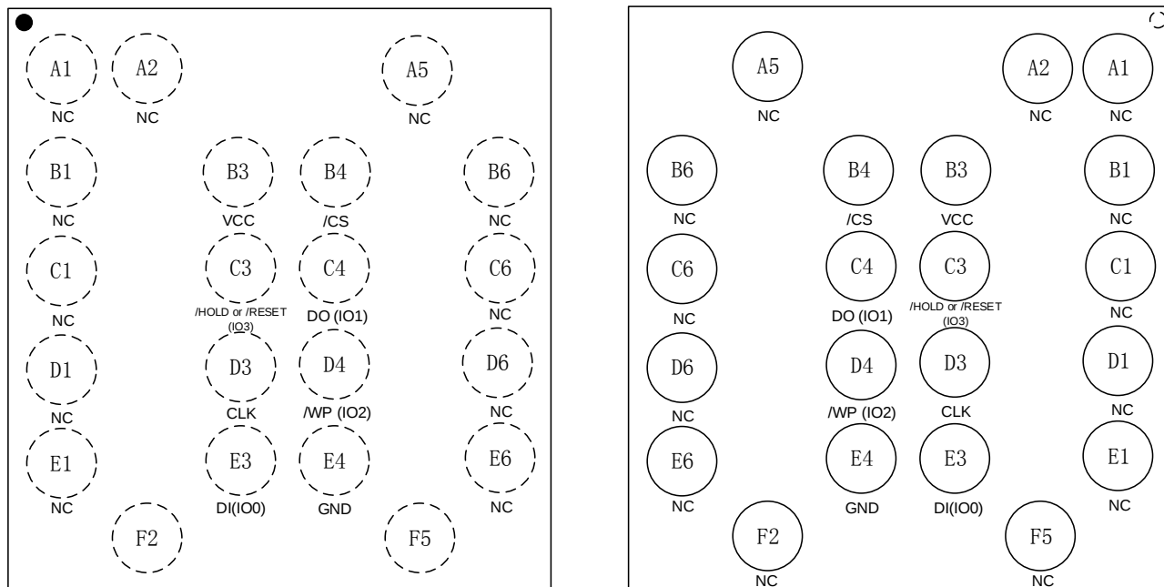
Figure 3.1f. WLCSP 21ball (Package Code V3)
