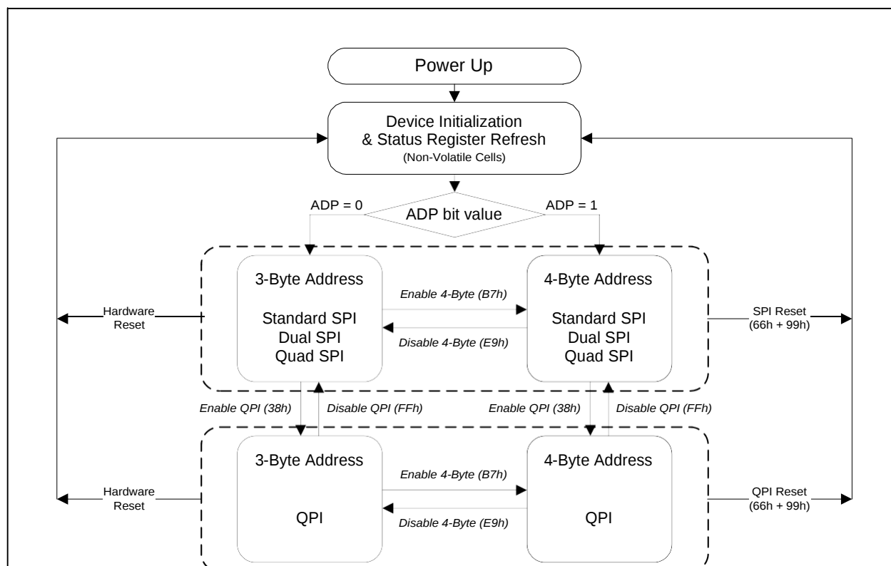
Figure 3. XM25QU256C Serial Flash Memory Operation Diagram
