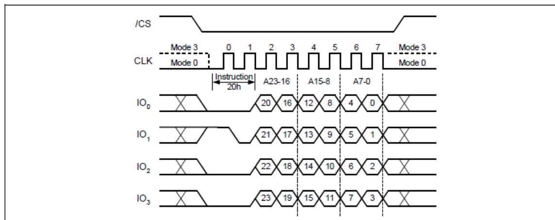
Figure 33b. Sector Erase Instruction (QPI Mode) 32-Bit Address is required when the device is operating in 4-Byte Address Mode
