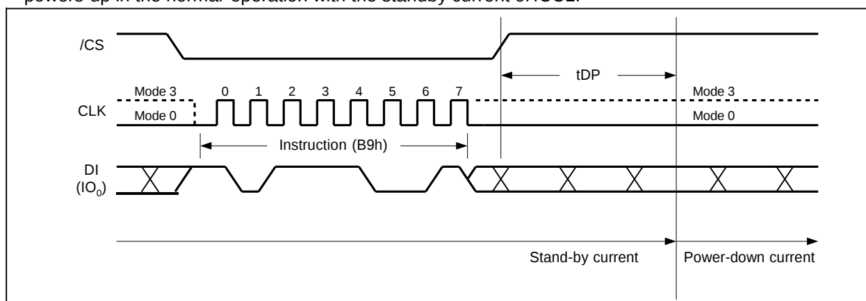
Figure 41a. Deep Power-down Instruction (SPI Mode)
