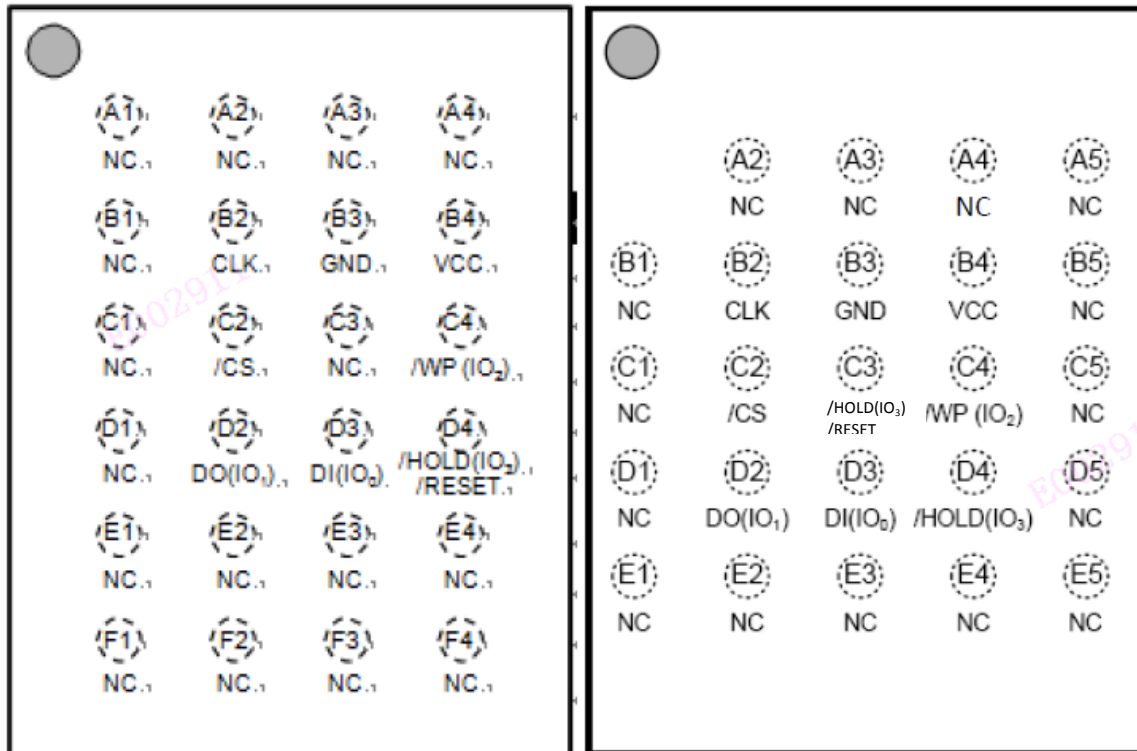
Figure 3.1d. XM25QU256C Ball Assignments, TFBGA 6x8 24ball (Package Code B,B2)
