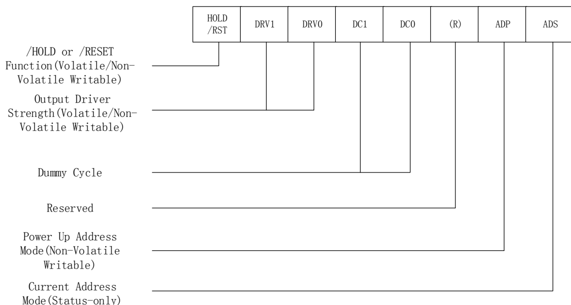
Figure 4c. Status Register-3
