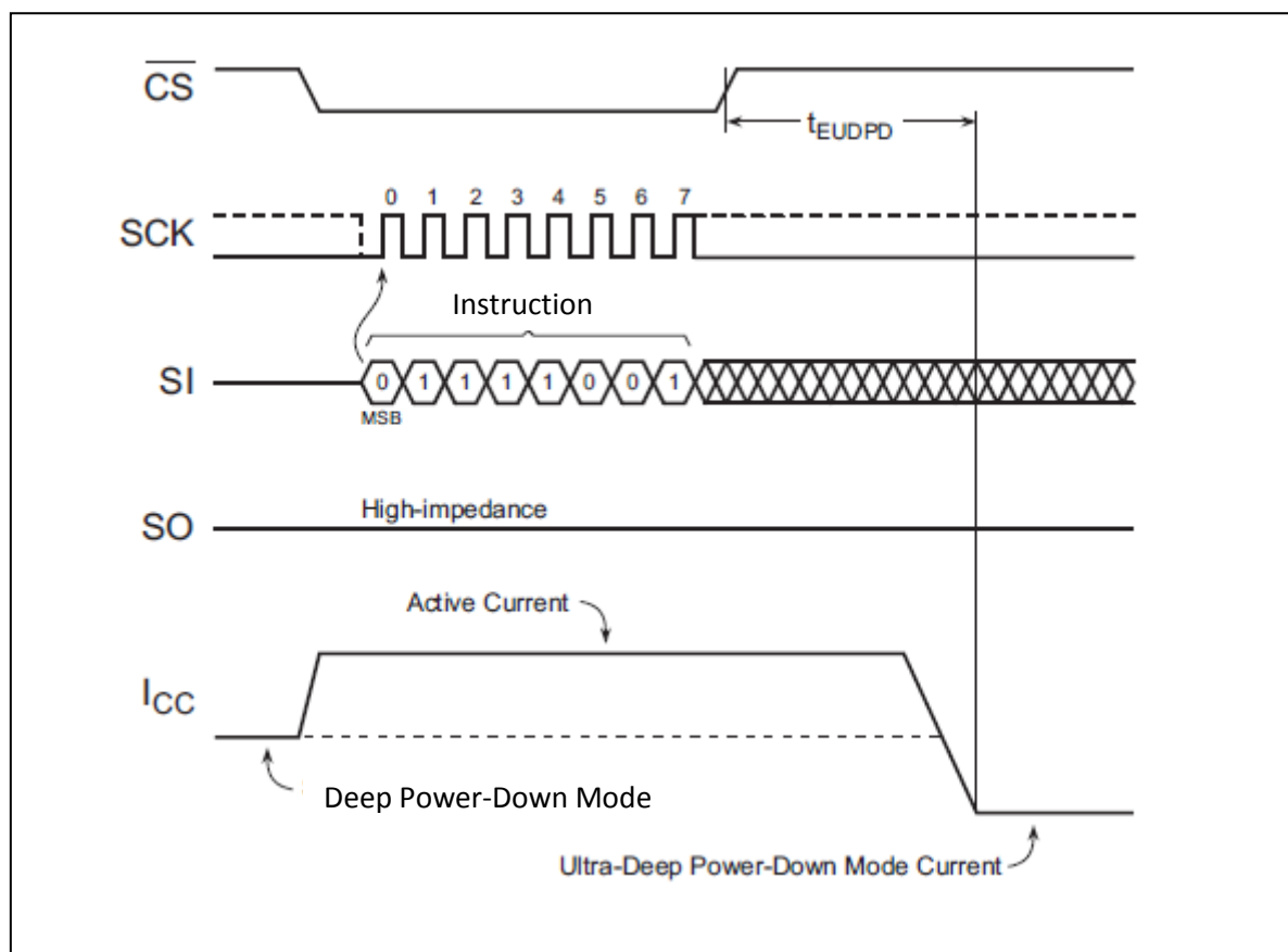
Figure 56. Ultra-Deep Power-Down
