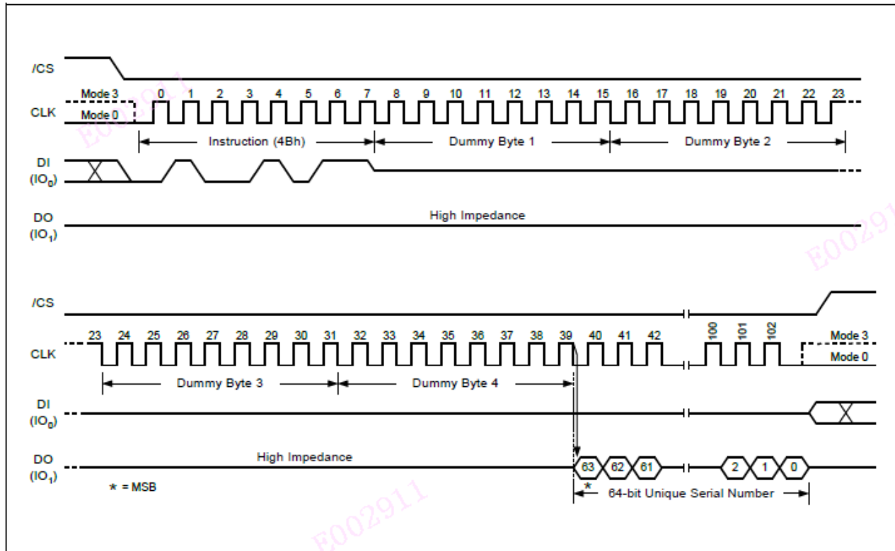
Figure 46. Read Unique ID Number Instruction (SPI Mode only)
