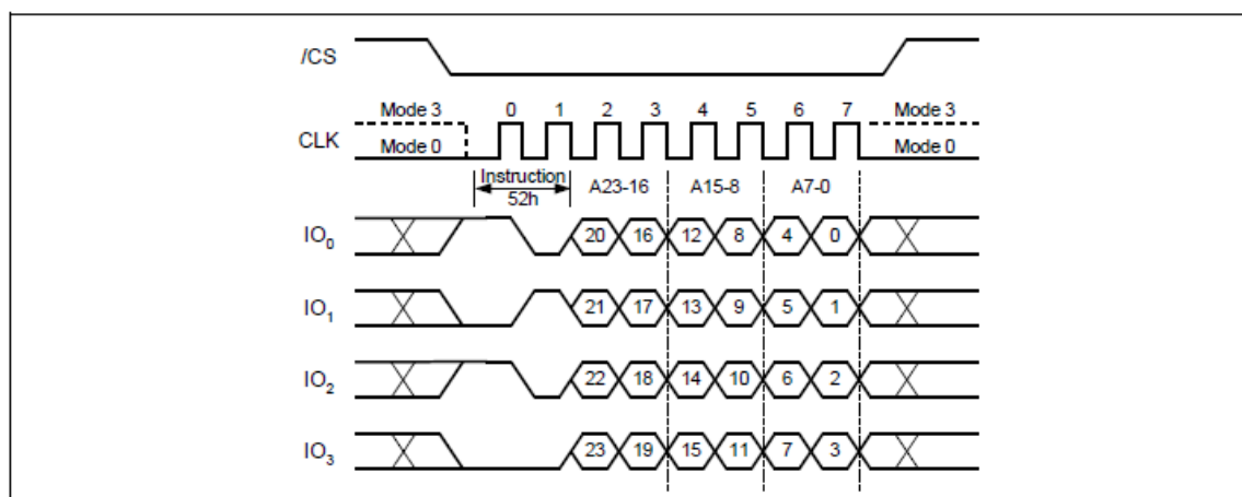
Figure 35b. 32KB Block Erase Instruction (QPI Mode)
