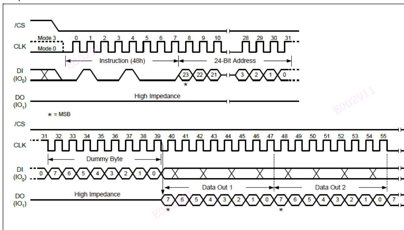
Figure 51. Read Security Registers Instruction (SPI Mode only) 32-Bit Address is required when the device is operating in 4-Byte Address Mode
