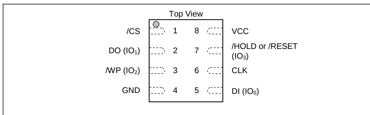
Figure 3.1a. XM25QU256C Pin Assignments, 8-pin SOP 208mil 8L (Package Code H)
