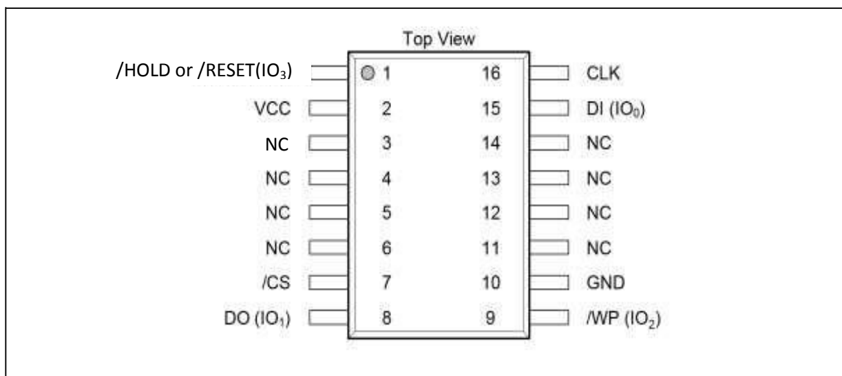
Figure 3.1c. XM25QU256C Pad Assignments, 16-pad SOP 300mil 16L (Package Code K)
