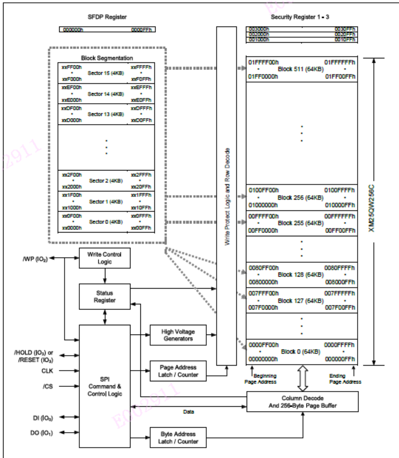
Figure 2. XM25QU256C Serial Flash Memory Block Diagram
