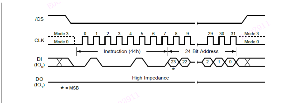
Figure 49. Erase Security Registers Instruction (SPI Mode only)
