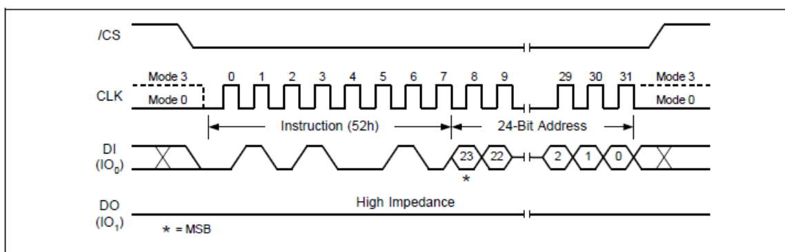
Figure 35a. 32KB Block Erase Instruction (SPI Mode)
