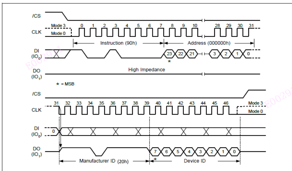
Figure 43. Read Manufacturer / Device ID Instruction (SPI Mode)
