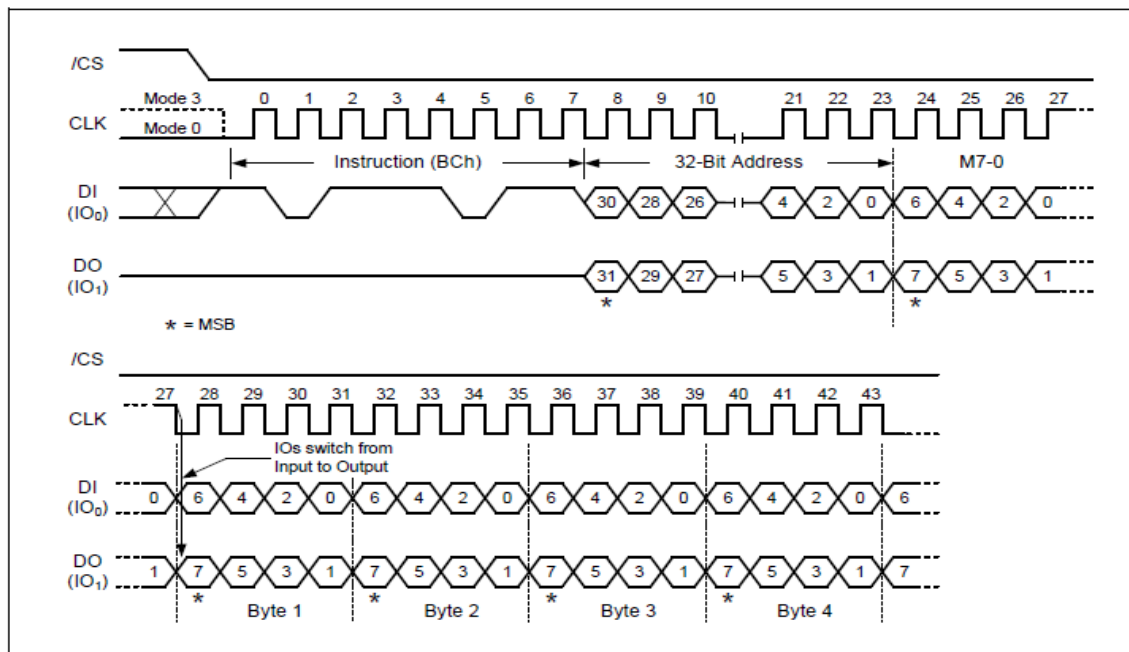
Figure 23a. Fast Read Dual I/O with 4-Byte Address Instruction. (Previous instruction set M5-4 \neq 10, SPI Mode only)
