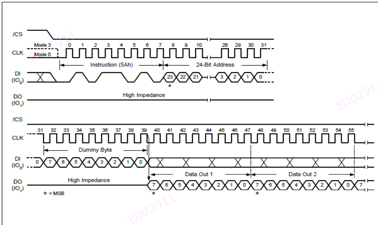
Figure 48. Read SFDP Register Instruction Sequence Diagram
