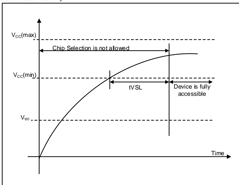
Figure 45a. Power-up Timing and Voltage Levels
